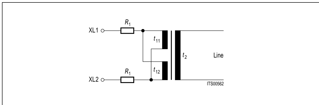
Figure 8 Transmitter Configuration
