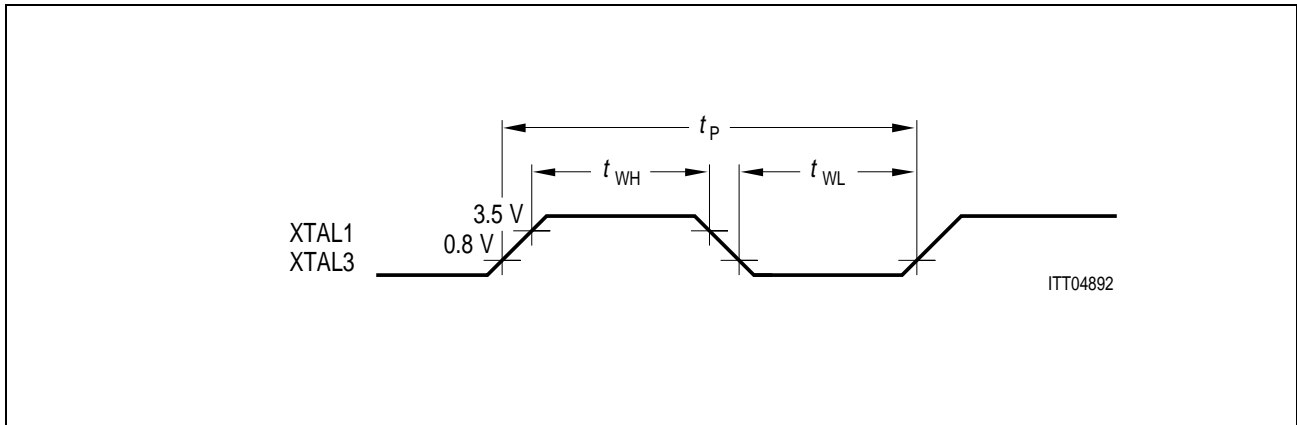
Figure 23 Timing of XTAL1/XTAL3
